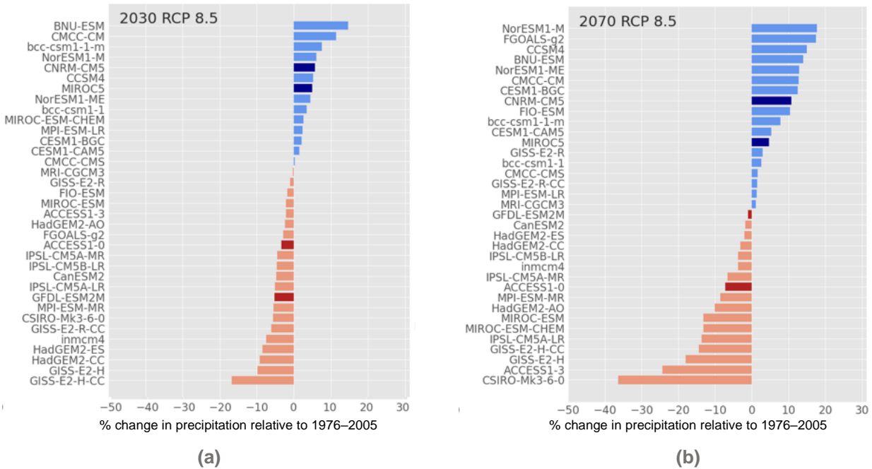
Figure 3.2. Ranking of the Monsoonal North region precipitation projections for the GCMs used in this study (shown in darker colours) compared to the CCiA ensemble for RCP8.5 for (a) 2030 and (b) 2070. The horizontal bars indicate the change signal – the difference of the regional average quantity from the monthly pattern for the reference period (1976–2005)
