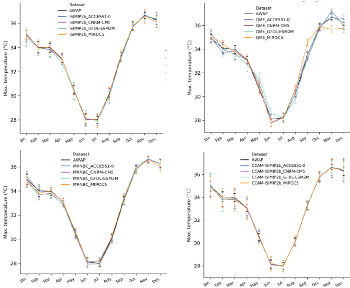
Figure 7.4. Comparison of the mean monthly maximum temperature (°C) for the 16-member ensemble and observed (AWAP) data for the Monsoonal North region (1976–2005)
