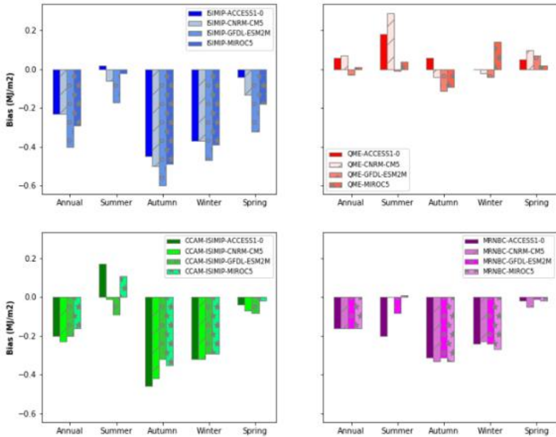
Figure 7.7. Bias (megajoules per square metre, MJ/m 2 ) in mean annual and seasonal solar radiation for the Monsoonal North region
