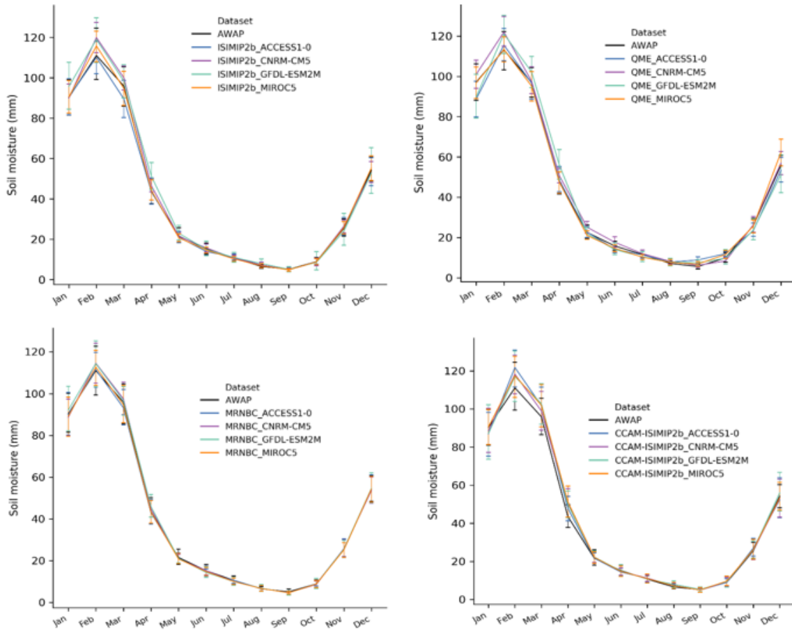
Figure 7.16. Comparison of the mean monthly soil moisture (mm) for the 16-member ensemble and observed (AWAP) data for the Monsoonal North region (1976–2005)
