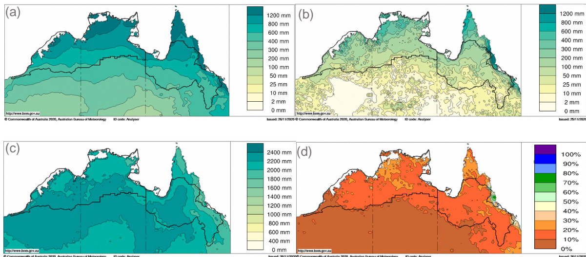
Figure 2.2. Monsoonal North annual average hydroclimate (1976–2005) showing (a) observed precipitation and AWRA-L modelled values for (b) runoff, (c) potential evapotranspiration and (d) soil moisture
