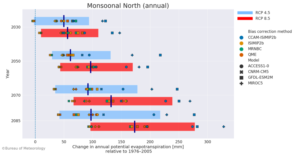
Figure 4.14. Absolute change (mm) in annual potential evapotranspiration projected by each ensemble member for 2030, 2050, 2070 and 2085 in the Monsoonal North region. The red bar shows the 10th to 90th percentiles for RCP8.5. The blue bar shows the 10th to 90th percentiles for RCP4.5. The dark blue line shows the ensemble median. The change is relative to the reference period (1976–2005)
