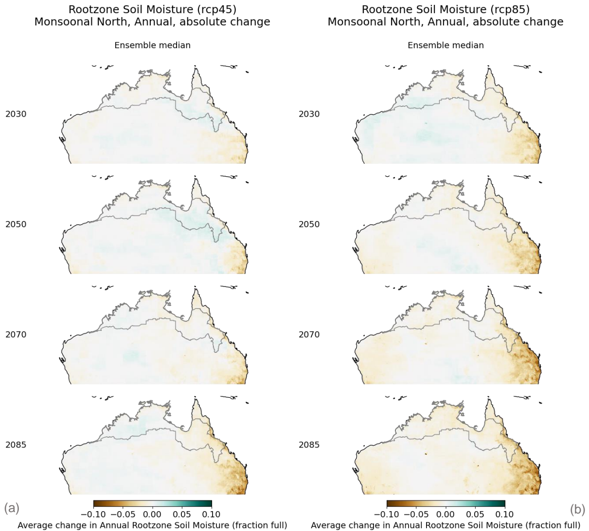
Figure 4.11. Absolute change (fraction full) (ensemble median) in annual modelled root zone soil moisture projected for 2030, 2050, 2070 and 2085 for (a) RCP4.5 and (b) RCP8.5 across the Monsoonal North region. The change is relative to the reference period (1976–2005). Fraction full (scale 0–1) is equivalent to (percentage full)/100 and represents the fraction of available water content in the root zone (0–1 m) soil profile
