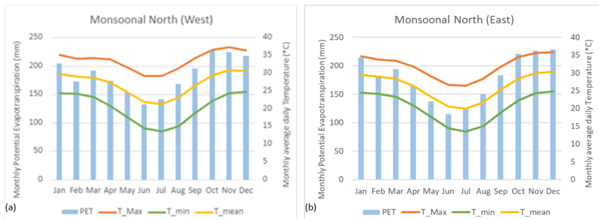
Figure 2.4. Monthly average observed maximum, minimum and mean temperature and AWRA-L modelled potential evapotranspiration for the (a) western and (b) eastern Monsoonal North subregions for the reference period (1976–2005)
