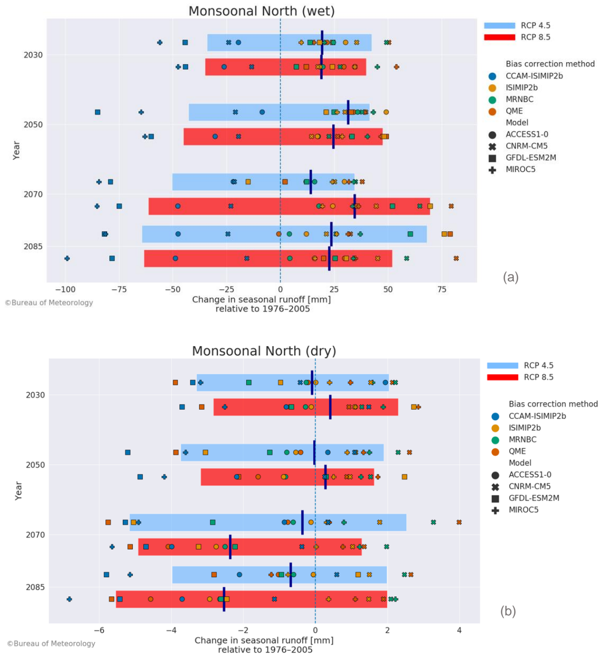
Figure 4.8. Absolute change (mm) projected by each ensemble member for (a) wet season (November–April) and (b) dry season (May–October) runoff for 2030, 2050, 2070 and 2085 in the Monsoonal North region. The red bar shows the 10th to 90th percentiles for RCP8.5. The blue bar shows the 10th to 90th percentiles for RCP4.5. The dark blue line shows the ensemble median. This change is relative to the reference period (1976–2005)
