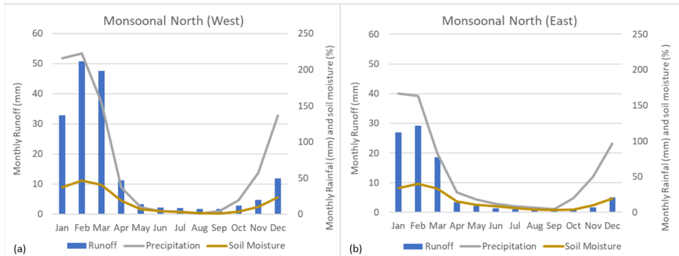
Figure 2.3. Monthly average observed precipitation and AWRA-L modelled runoff and soil moisture for (a) western and (b) eastern Monsoonal North subregions for the reference period (1976–2005)
