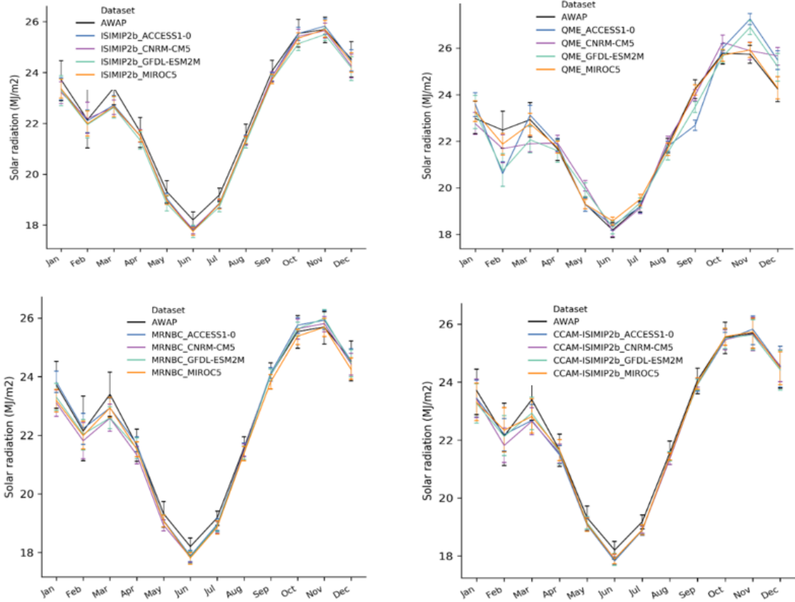
Figure 7.8. Comparison of the mean monthly solar radiation (MJ/m 2 ) for the 16-member ensemble and observed (AWAP) data for the Monsoonal North region (1976–2005)
