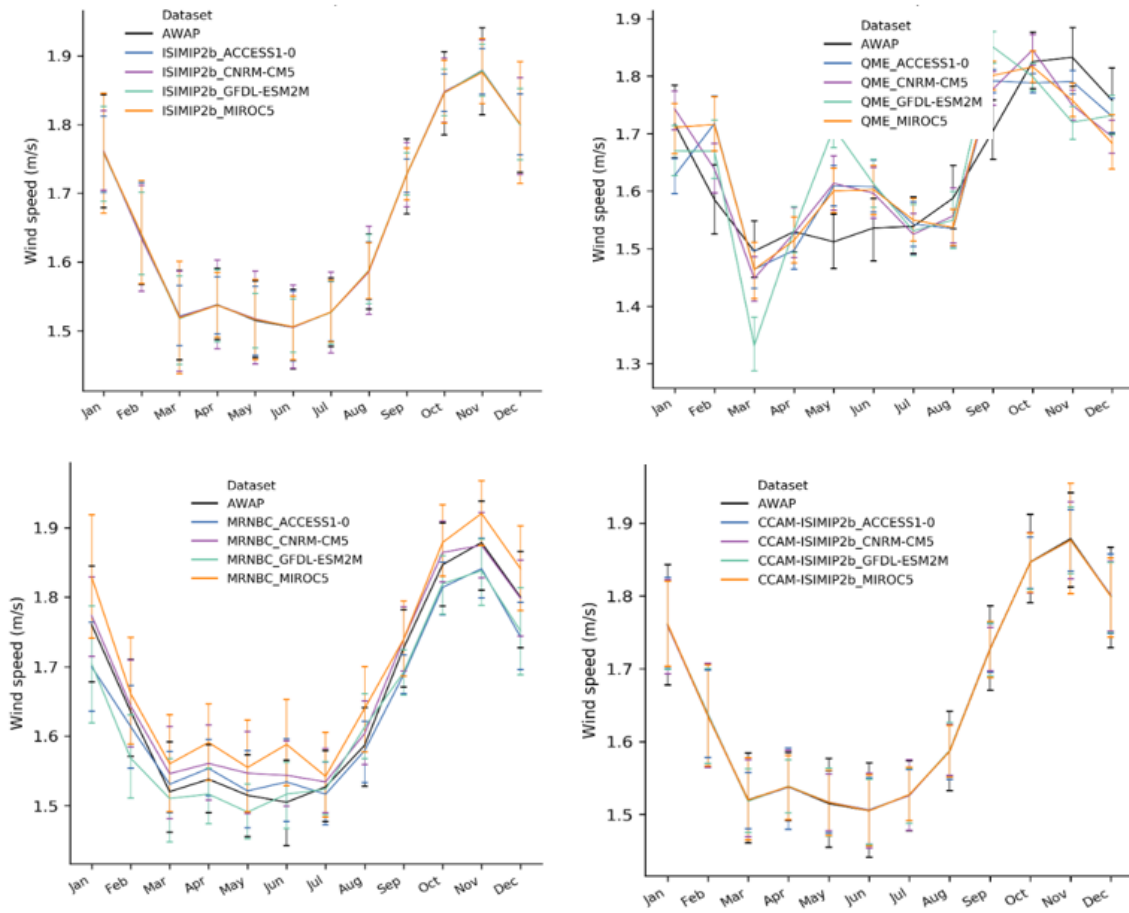
Figure 7.10. Comparison of the mean monthly wind speed (m/s) for the 16-member ensemble and observed (AWAP) data for the Monsoonal North region (1976–2005)
