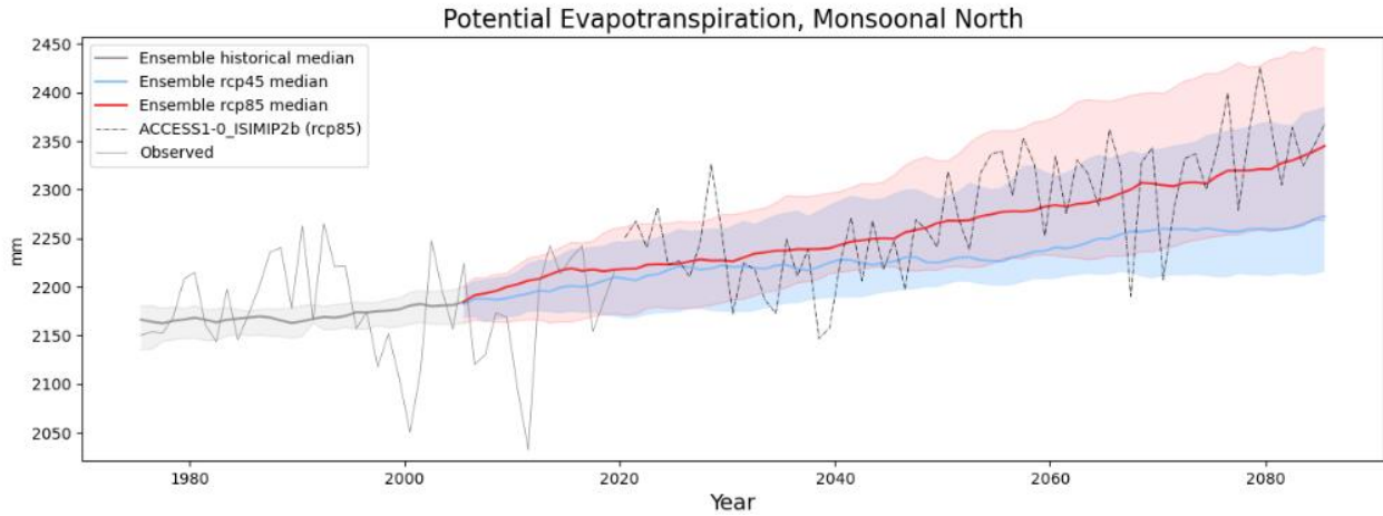
Figure 4.13. Annual modelled potential evapotranspiration (mm) projected to 2099 by ensemble members for RCP4.5 (blue) and RCP8.5 (red) in the Monsoonal North region. The shaded areas represent the 10th to 90th percentile range for all ensemble members in the historical and future time periods. The time series for ACCESS1-0_ISIMIP2b (RCP8.5) is included (dotted line) to show the variability projected for an individual ensemble member. The grey line represents the modelled historical median potential evapotranspiration
