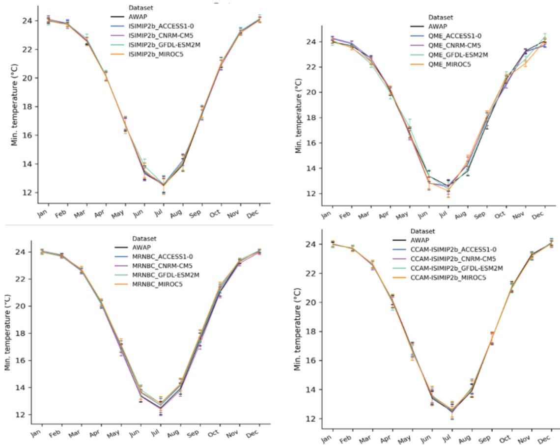
Figure 7.6. Comparison of the mean monthly minimum temperature (°C) for the 16-member ensemble and observed (AWAP) data for the Monsoonal North region (1976–2005)
