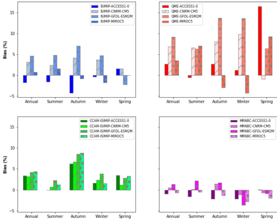
Figure 7.15. Bias (%) in mean annual and seasonal soil moisture for the Monsoonal North region
