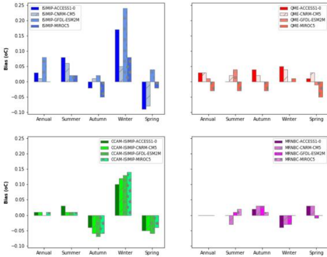
Figure 7.5. Bias (°C) in mean annual and seasonal minimum temperature for the Monsoonal North region
