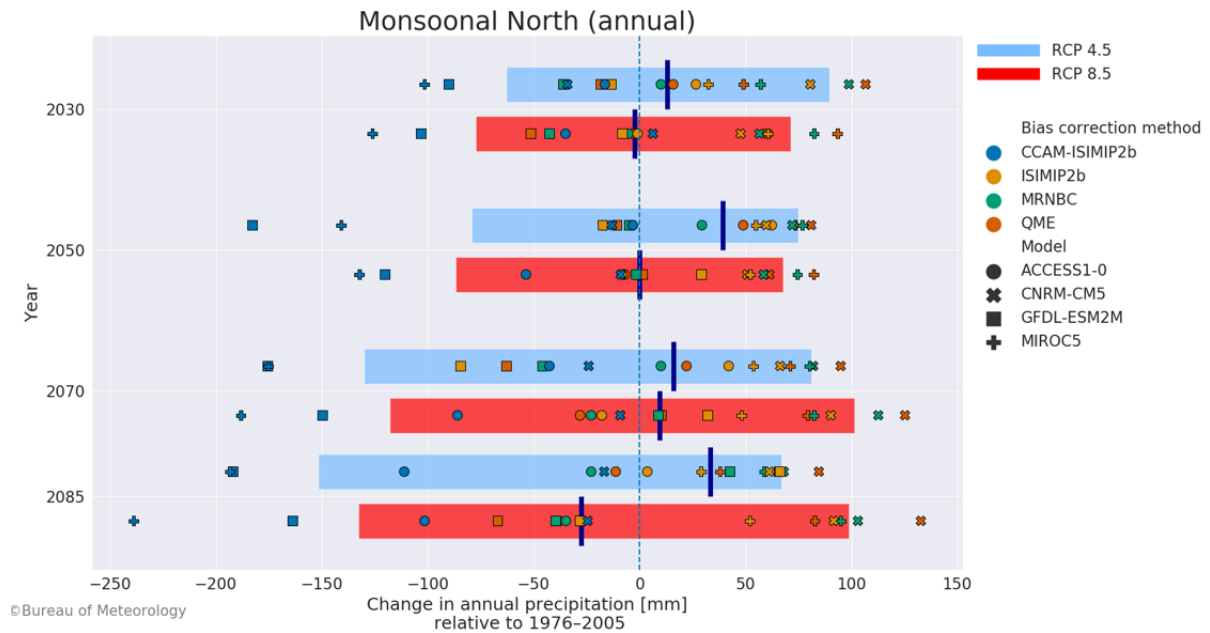
Figure 4.2. Change in annual precipitation (mm) projected by each ensemble member for 2030, 2050, 2070 and 2085 in the Monsoonal North region. The red bar shows the 10th to 90th percentiles for RCP8.5. The blue bar shows the 10th to 90th percentiles for RCP4.5. The dark blue line shows the ensemble median. The change is relative to the reference period (1976–2005)
