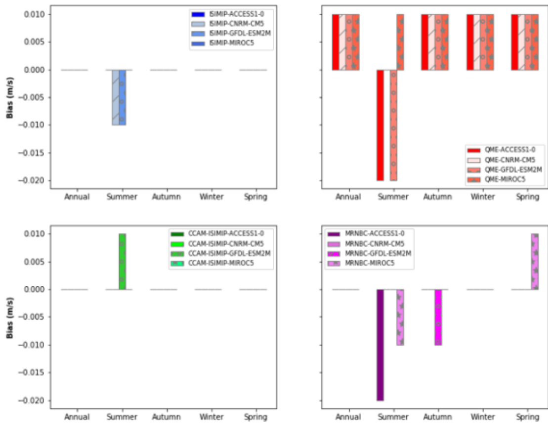
Figure 7.9. Bias (m/s) in mean annual and seasonal wind speed for the Monsoonal North region
