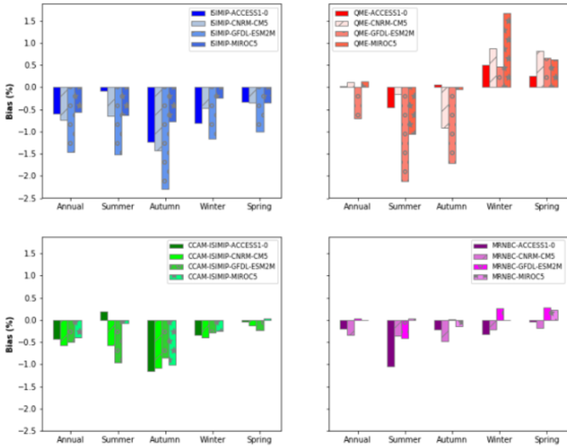
Figure 7.13. Bias (%) in mean annual and seasonal potential evapotranspiration for the Monsoonal North region
