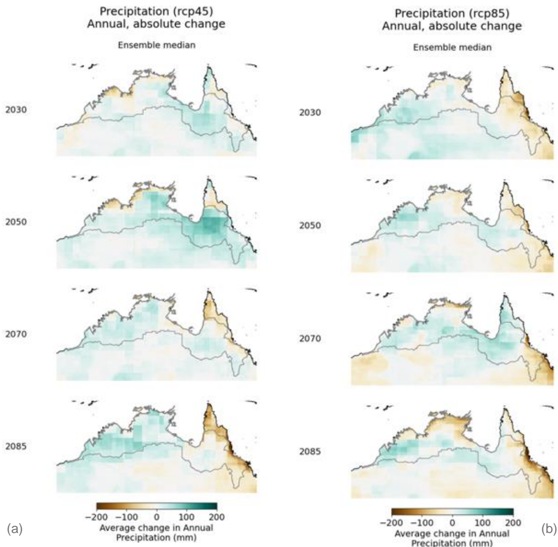
Figure 4.3. Absolute change (mm) (median) in annual modelled precipitation projected across the Monsoonal North region for 2030, 2050, 2070 and 2085 for (a) RCP4.5 and (b) RCP8.5. The change is relative to the reference period (1976–2005)
