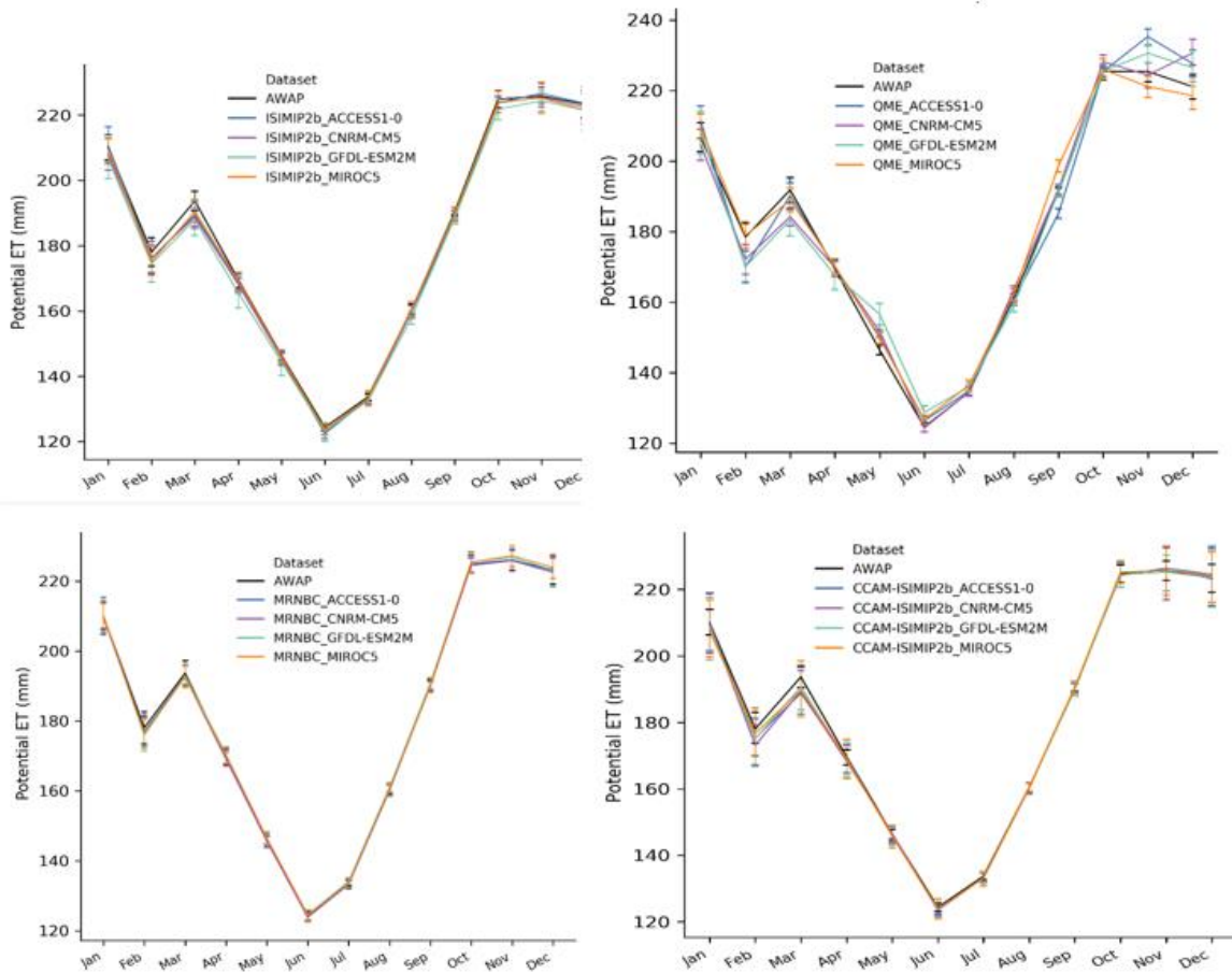
Figure 7.14. Comparison of the mean monthly potential evapotranspiration (mm) for the 16-member ensemble and observed (AWAP) data for the Monsoonal North region (1976–2005)
