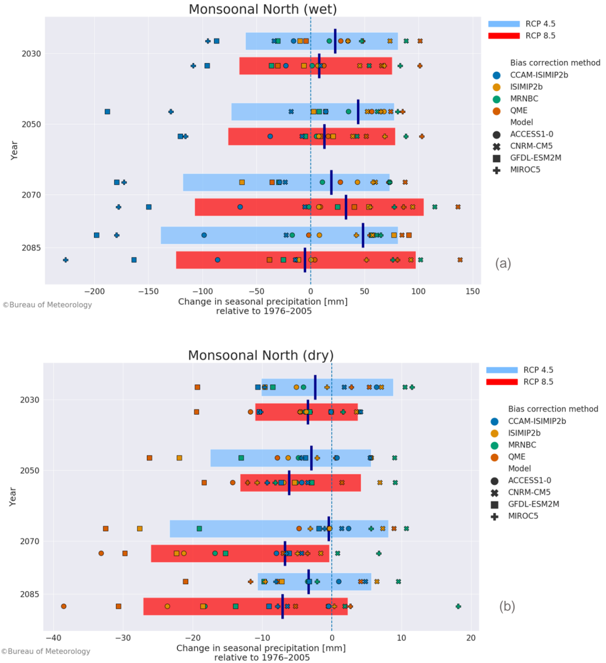
Figure 4.4. Absolute change in modelled precipitation (mm) projected by each ensemble member for (a) wet season (November–April) and (b) dry season (May–October) for 2030, 2050, 2070 and 2085 in the Monsoonal North region. The red bar shows the 10th to 90th percentiles for RCP8.5. The blue bar shows the 10th to 90th percentiles for RCP4.5. The dark blue line shows the ensemble median. The change is relative to the reference period (1976–2005)
