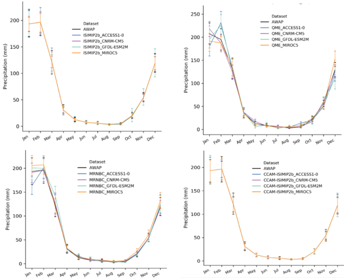
Figure 7.2. Comparison of the mean monthly precipitation (mm) for the 16-member ensemble and observed (AWAP) data of the Monsoonal North region (1976–2005)
