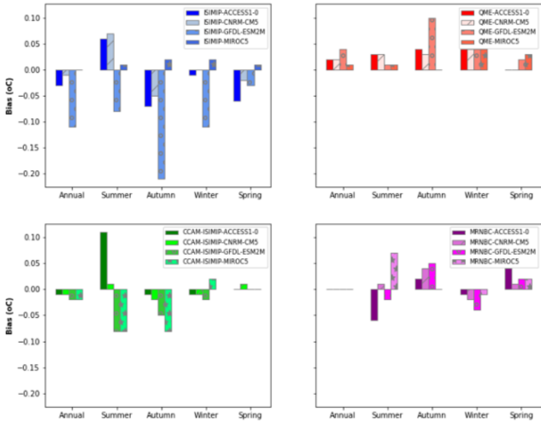
Figure 7.3. Bias (°C) in mean annual and seasonal maximum temperature for the Monsoonal North region
