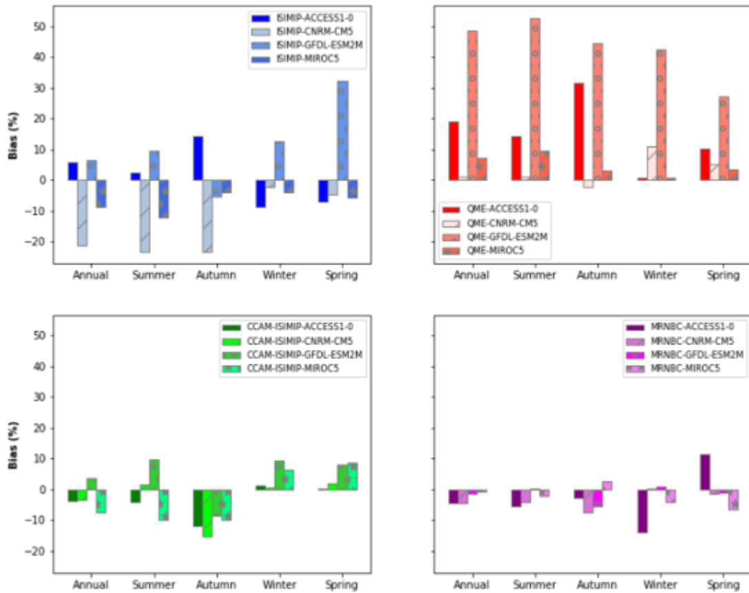
Figure 7.11. Bias (%) in mean annual and seasonal runoff for the Monsoonal North region
