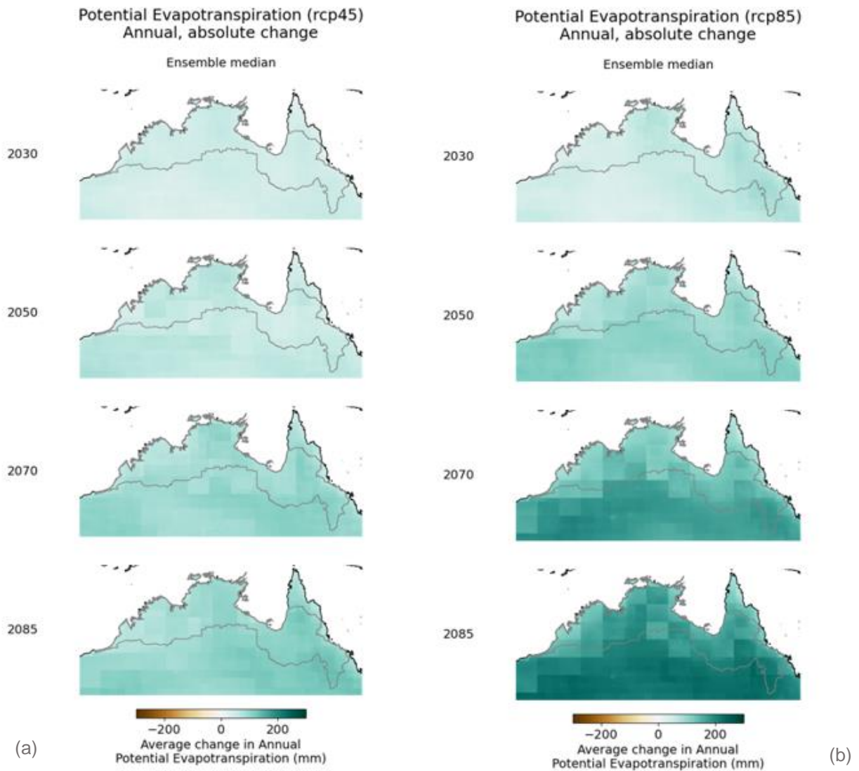
Figure 4.15. Absolute change (mm) (ensemble median) in annual modelled potential evapotranspiration for (a) RCP4.5 and (b) RCP8.5 for 2030, 2050, 2070 and 2085 across the Monsoonal North region. The change is relative to the reference period (1976–2005)
