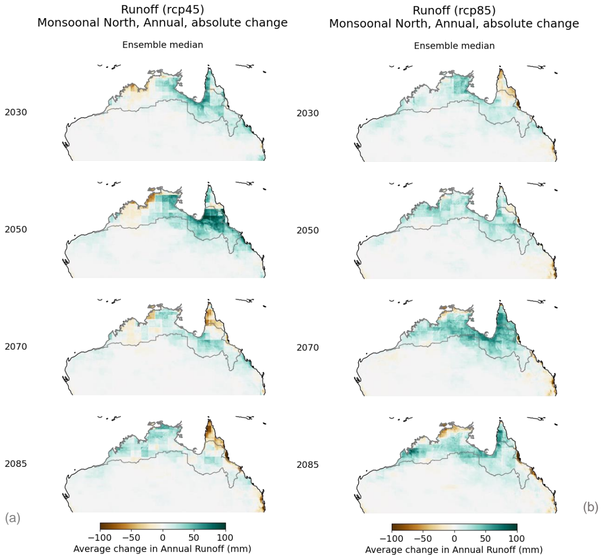
Figure 4.7. Absolute change (mm) (median) in annual modelled runoff projected across the Monsoonal North region for 2030, 2050, 2070 and 2085 for (a) RCP4.5 and (b) RCP8.5. This change is relative to the reference period (1976–2005)
