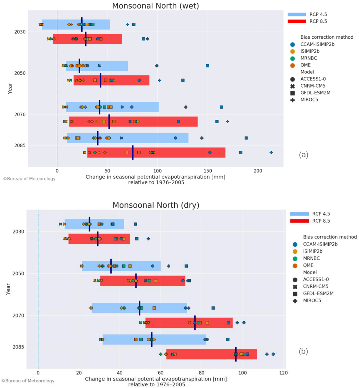
Figure 4.16. Absolute change (mm) in potential evapotranspiration projected by each ensemble member for (a) wet season (November–April) and (b) dry season (May–October) for 2030, 2050, 2070 and 2085 in the Monsoonal North region. The red bar shows the 10th to 90th percentiles for RCP8.5. The blue bar shows the 10th to 90th percentiles for RCP4.5. The dark blue line shows the ensemble median. The change is relative to the reference period (1976–2005)
