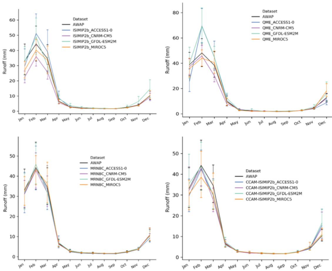
Figure 7.12. Comparison of the mean monthly runoff (mm) for the 16-member ensemble and observed (AWAP) data for the Monsoonal North region (1976–2005)
