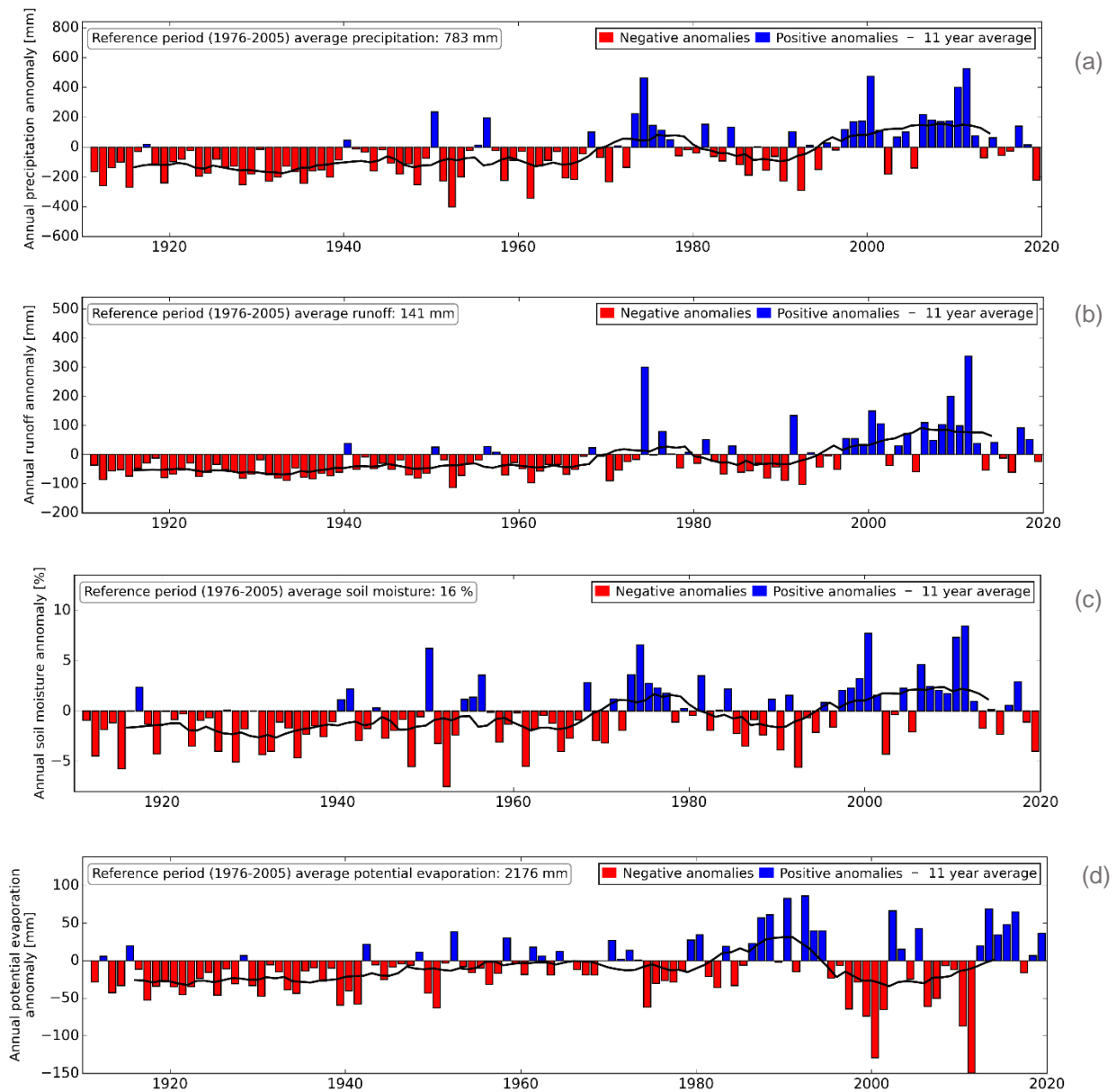
Figure 2.5. Monsoonal North annual anomalies relative to the reference period (1976–2005) mean in (a) observed precipitation and AWRA-L modelled values for (b) runoff, (c) soil moisture and (d) potential evapotranspiration
