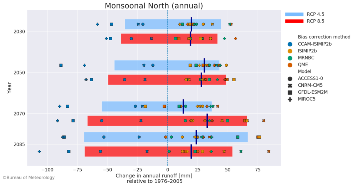
Figure 4.6. Absolute change in annual runoff (mm) projected by each ensemble member for 2030, 2050, 2070 and 2085 in the Monsoonal North region. The red bar shows the 10th to 90th percentiles for RCP8.5. The blue bar shows the 10th to 90th percentiles for RCP4.5. The dark blue line shows the ensemble median. The change is relative to the reference period (1976–2005)
