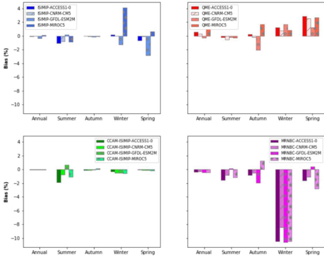
Figure 7.1. Bias (%) in mean annual and seasonal precipitation for the 16-member ensemble and observed (AWAP) data of the Monsoonal North region
