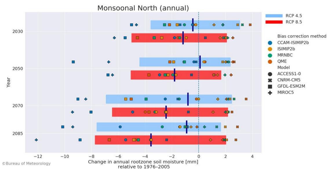
Figure 4.10. Absolute change (mm) in annual root zone soil moisture projected by each ensemble member for 2030, 2050, 2070 and 2085 in the Monsoonal North region. The red bar shows the 10th to 90th percentiles for RCP8.5. The blue bar shows the 10th to 90th percentiles for RCP4.5. The dark blue line shows the ensemble median. The change is relative to the reference period (1976–2005)
